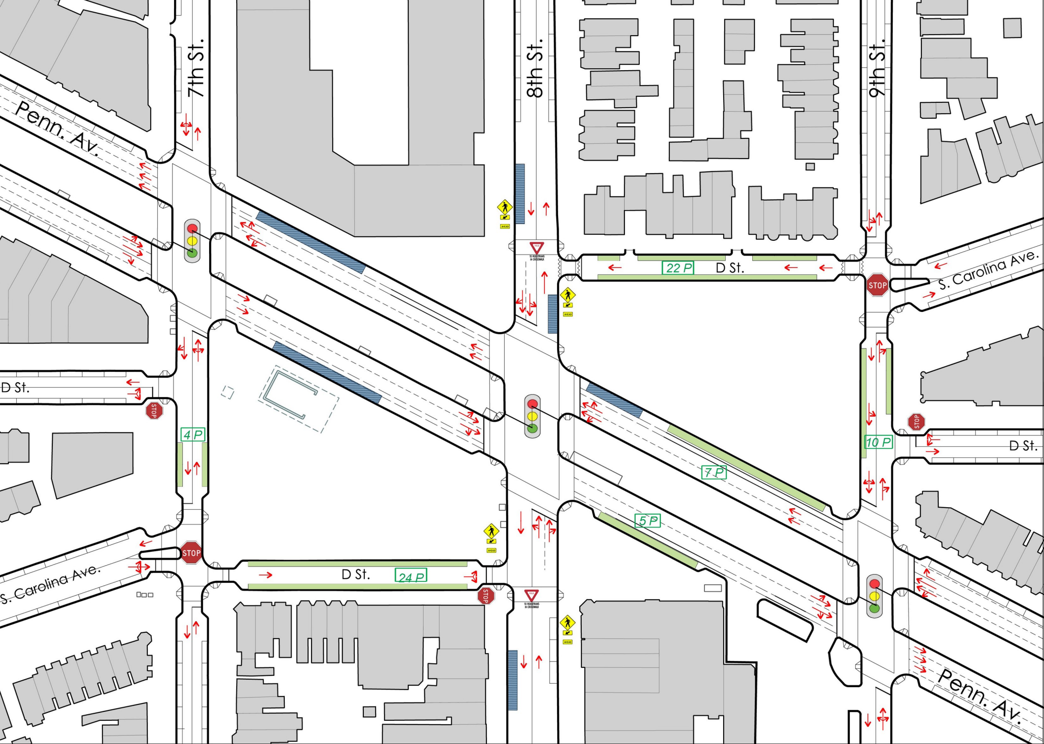
Existing (Improved) Traffic Diagram
